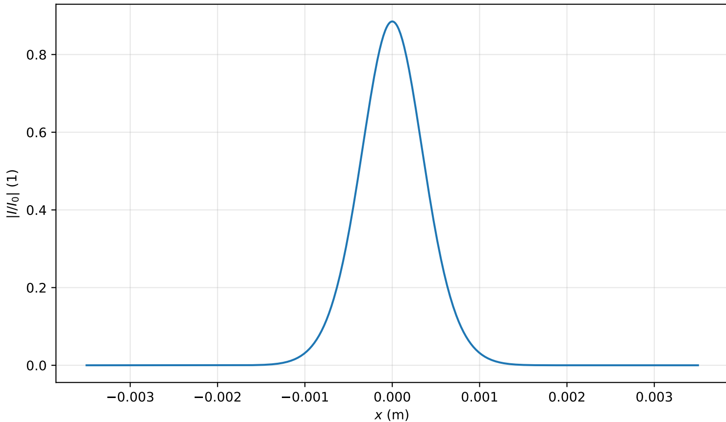
Intensity profile I(x, y = 0, z = 1.194m)/I_0 , P_{in}=0.3P_{cr} , artificial time
